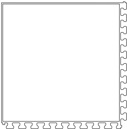
Fliese 500 x 500 x 7 mm
